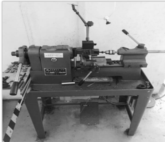
Gauge Lathe [1]
